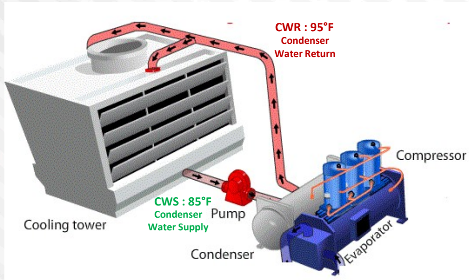
Cooling Tower / Condenser Water – Open Circuit
