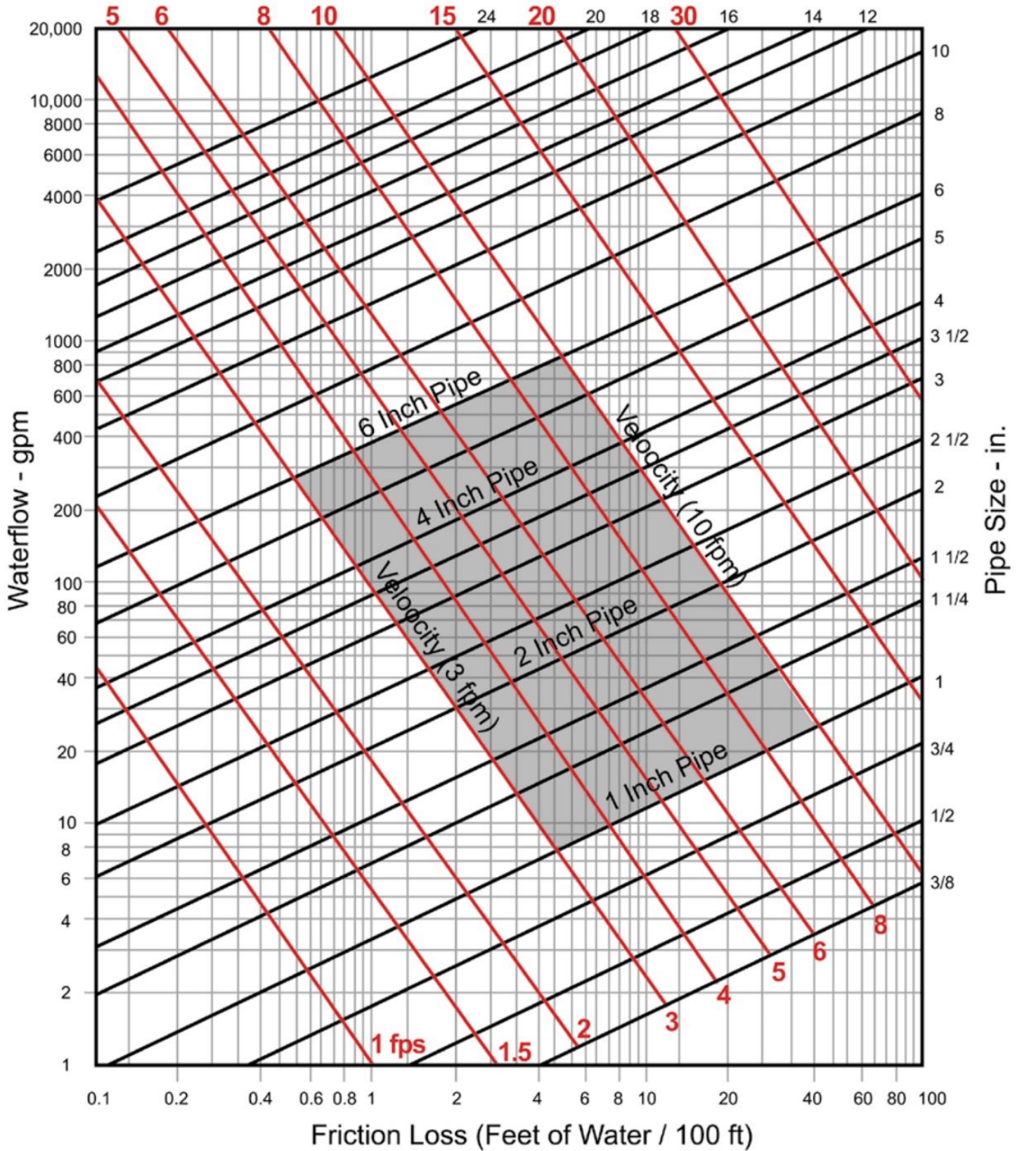
Chart 1 - Friction Loss for Closed-Loop System Schedule 40 Steel
